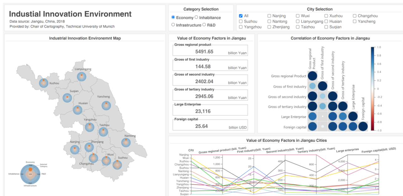
Figure 1. The layout of an interactive map-based dashboard used in our experiment.
